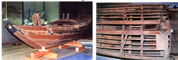
Fig.4 'Kompira-maru', dedicated model to Kotohira-gu
