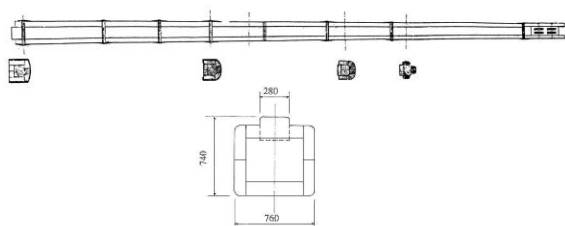
Fig. 7 Main mast called 'Taimatsu-bashira'
