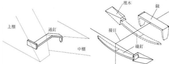
Fig. 8 Nails used for Naniwa-maru
