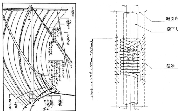
Fig.6 Assembly of sail (left: from the document of Edo era, right: assembly plan for 'Naniwa-maru')
