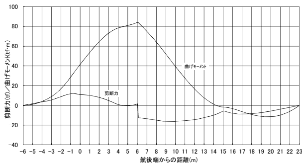
Fig.14 Bending moment / shearing force diagram (full load)
