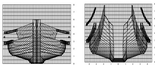
Fig.3 Lines of 'Naniwa-maru'
