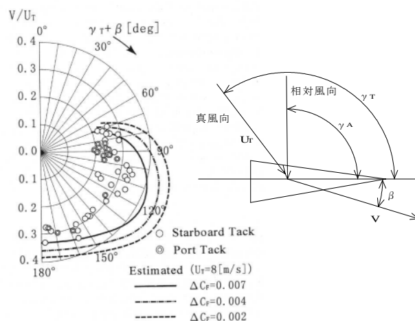
Fig.13 Polar diagram obtained by sea trial
