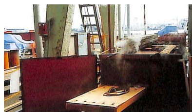
Fig. 9 Steam box for bending shell plates
