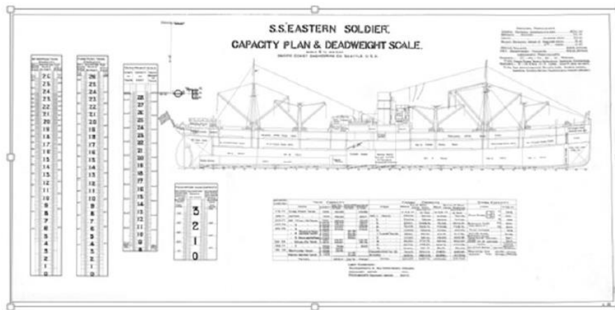
(FIG-11) Capacity Plan & Deadweight Scale
